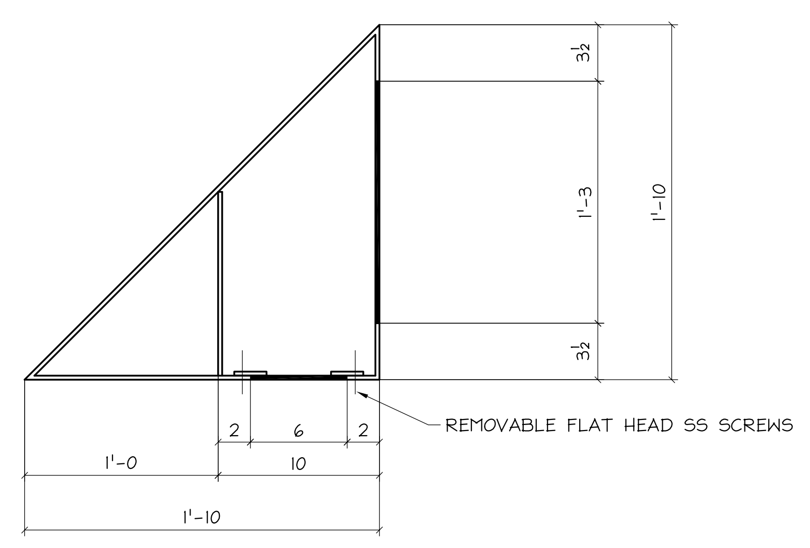
SECT-B
